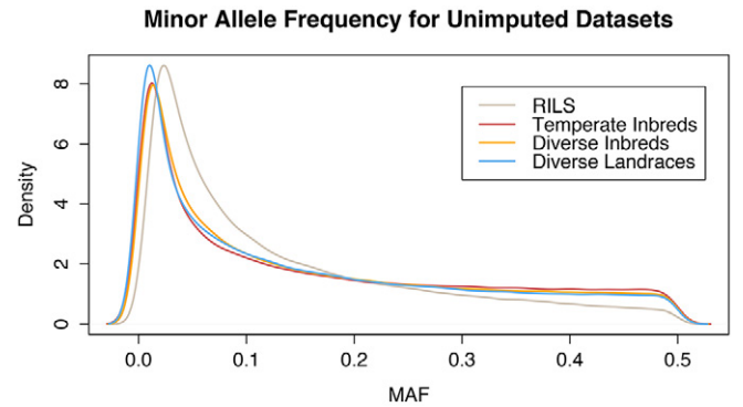
Figure 4. Minor allele frequency (MAF) densities for the unimputed datasets used for this study. For the recombinant inbred lines (RILs), the MAF was calculated in each biparental family separately, and combined. Populations sizes are as follows: temperate inbreds (429), diverse inbreds (367), diverse landraces (366), nested association mapping RILs (4667).
