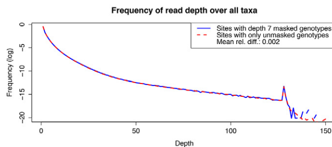
Figure 3. Sites that contain masked genotypes show the same read depth distribution as sites without masked genotypes, suggesting that masked genotypes are representative and acceptable for calculating accuracy.
