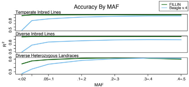
Figure 8. Accuracy for sites with different minor allele frequencies (MAF). The MAF for Fast Inbred Line Library ImputationN (FILLIN) is taken from the donor haplotype files, while the MAF for Beagle v. 4 and Fast Inbred Line Library ImputationN is taken from the unimputed input data.
