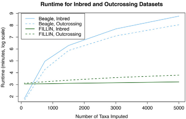
Figure 9. Computational time for Fast Inbred Line Library ImputationN (FILLIN) and Beagle v. 4. Only one chromosome (chromosome 10) was compared, since computing the whole genome with >1000 samples using Beagle v. 4 is intractable unless parallelized. Each subset is a random sample of the larger taxa set.
