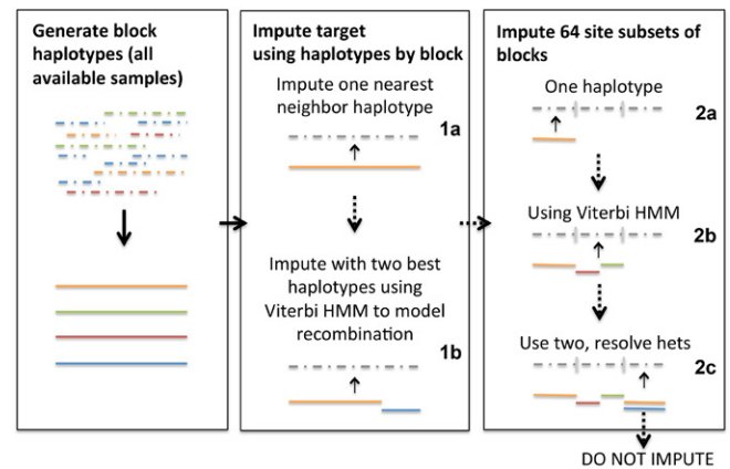
Figure 2. Fast Inbred Line Library ImputationN (FILLIN) algorithm overview. FILLIN first tries to impute the entire site window with one (1a) or two (1b) haplotypes (using the Viterbi Hidden Markov Model [HMM] to model the recombination break point), then if that is unsuccessful tries to impute for smaller windows, first with one haplotype (2a), then two with Viterbi (2b), finally by combining two haplotypes to model heterozygosity (2c). If this does not satisfy (lower) error thresholds, the smaller window is not imputed. Refer to methods for detailed description of 1a–2c. Dashed arrows mean that the algorithm continues if conditions are not satisfied for imputation.
